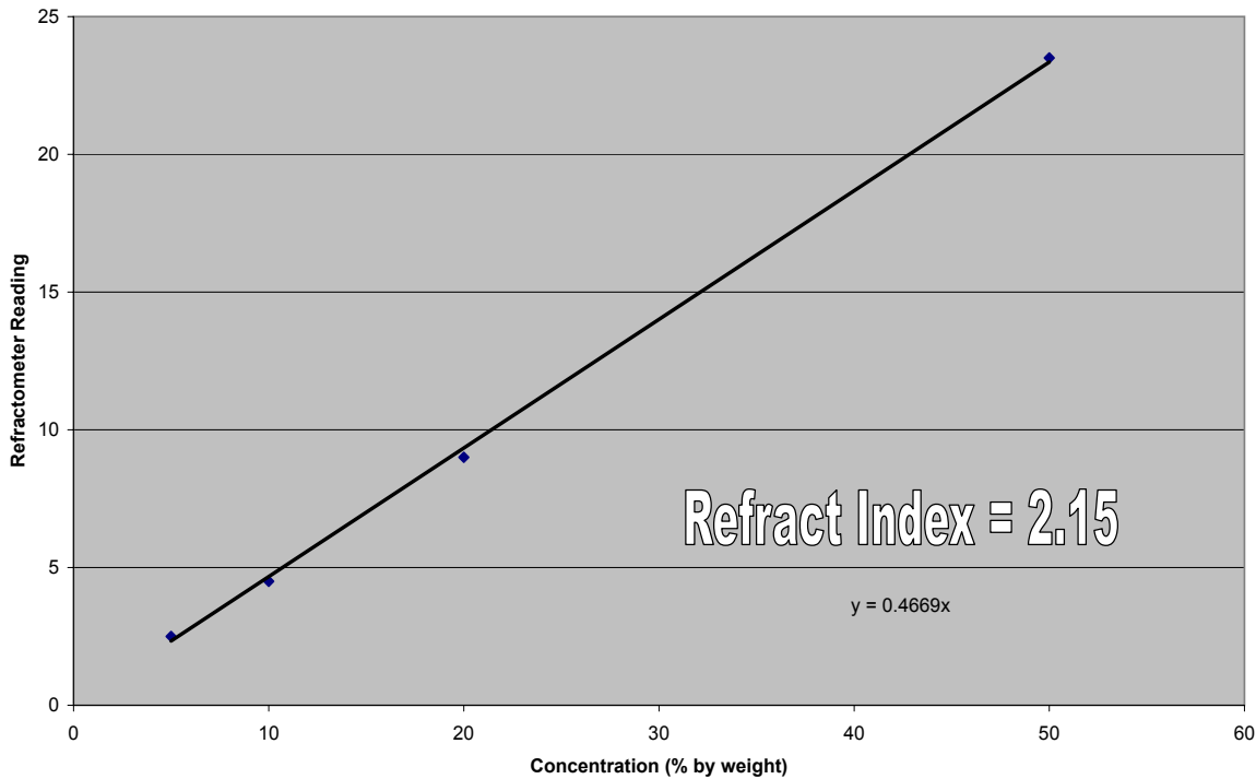
Refractometer Curve for VpCI-379
